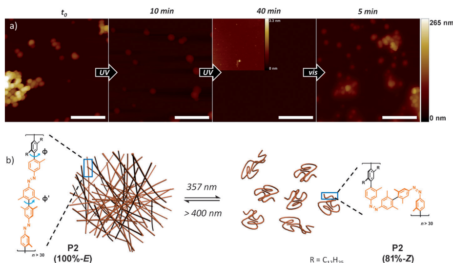
Figure 3. Light induced reversible disruption of molecular aggregates of P2 ( R = C_{12}H_{25} ). a) Selected snapshots of the disruption process (SFM), scale bar: 1 \mu\text{m} . The inset ( t = 40 min) shows a z-expansion (z-scale: 3.3 nm) of the surface, emphasizing the absence of aggregates after UV-light irradiation. The aggregates were spin-coated on mica from a 1 \text{ g L}^{-1} solution of P2 in THF. b) Polymer P2 contains a few solubilizing groups and therefore aggregates in the extended (100%-E) state. In the compressed (81%-Z) state, the intermolecular aggregates are disrupted.
